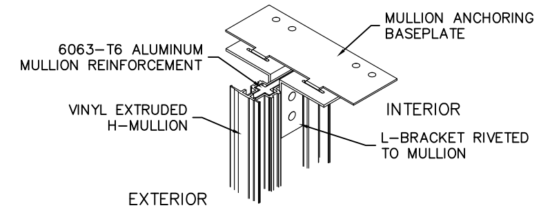
MULLION DETAIL
